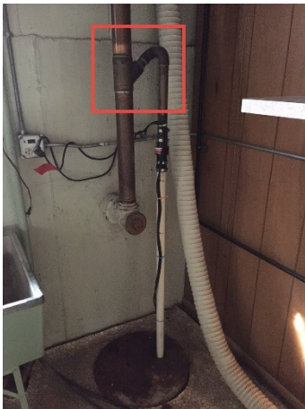
Figure 7 Illegal Sump Pump Connection
