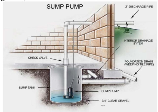
Figure 8 LEGAL Sump Pump Connection
